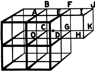
FIG. 1.—Simple cubic lattice of valence electrons of a fictitious univalent element.
